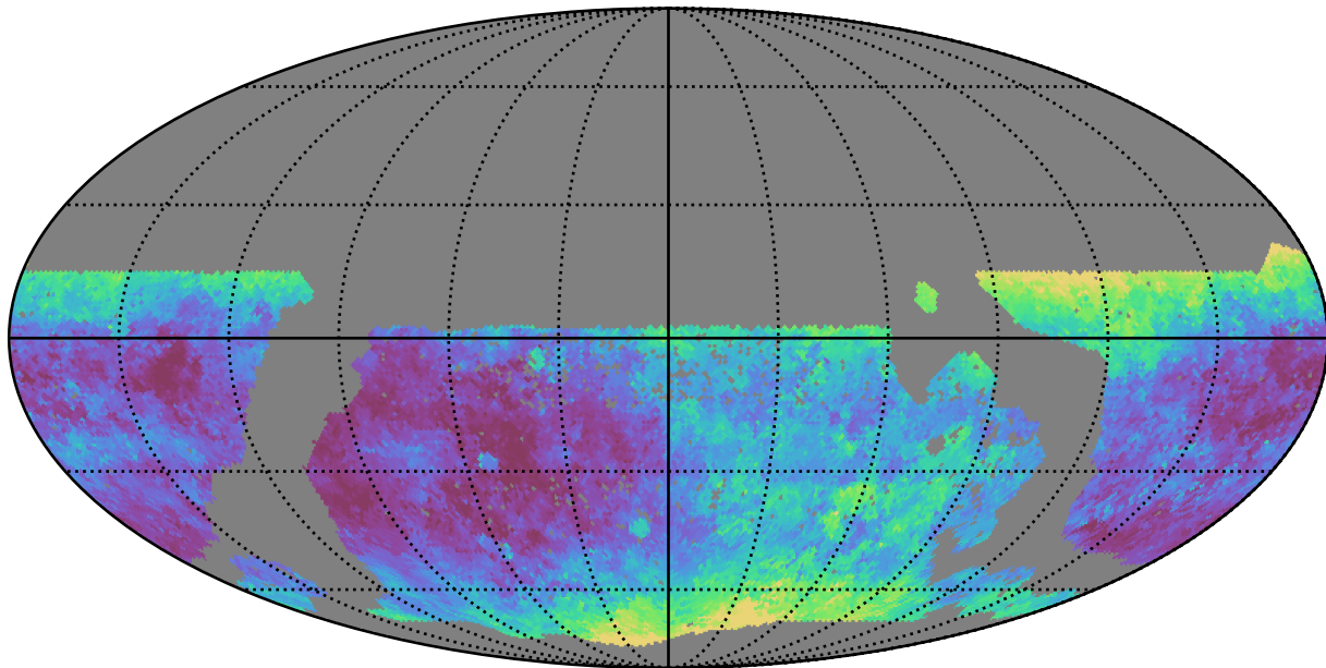
mw_roll_bulge_v3.3_10yrs WFD g band: Median seeingEff
