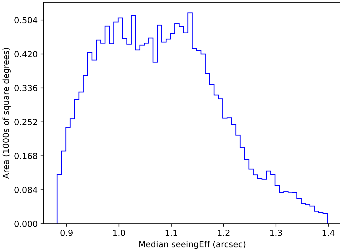
mw_roll_bulge_v3.3_10yrs WFD g band: Median seeingEff
