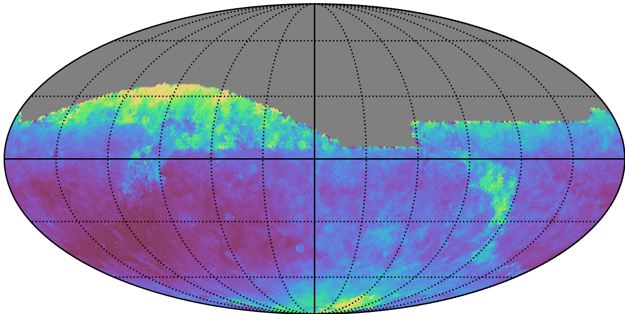
mw_roll_bulge_v3.3_10yrs All sky z band: Median seeingEff
