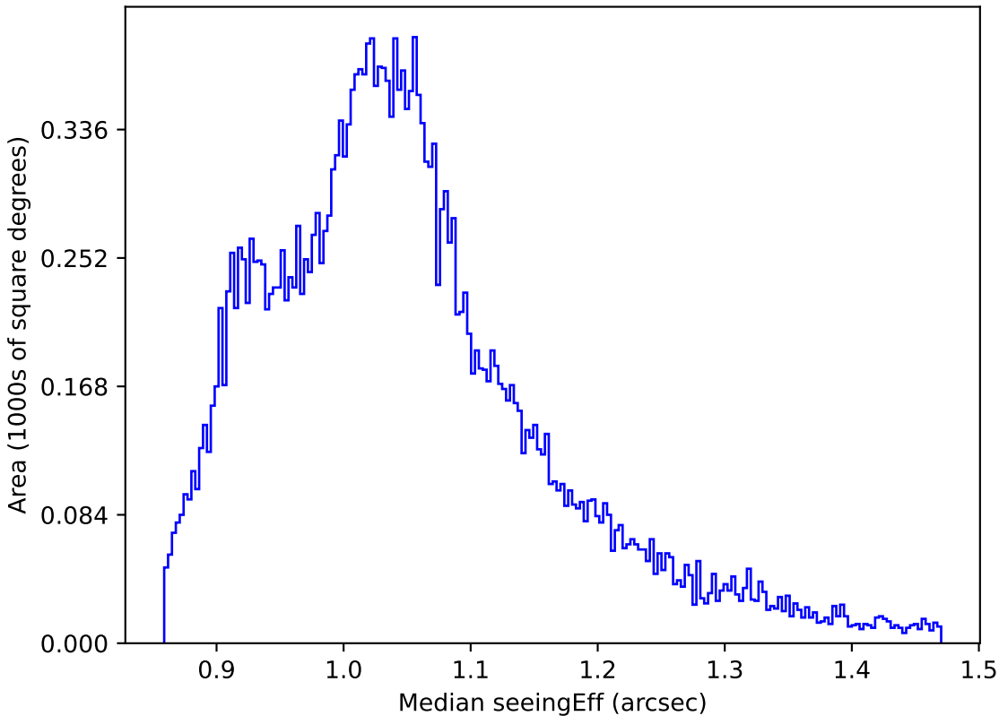
mw_roll_bulge_v3.3_10yrs All sky z band: Median seeingEff
