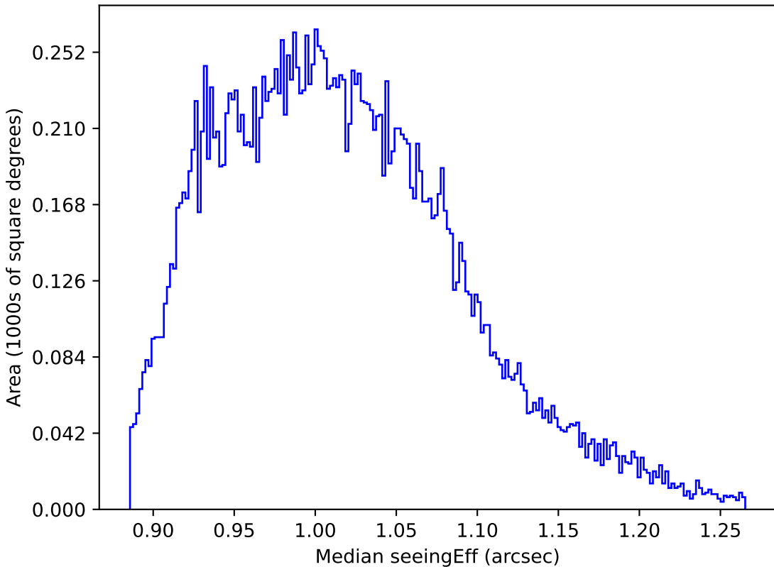
mw_roll_bulge_v3.3_10yrs All sky y band: Median seeingEff
