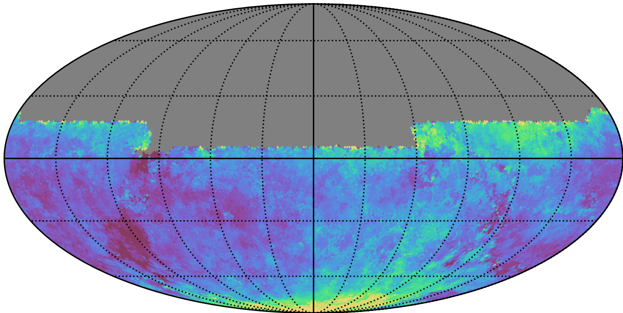
mw_roll_bulge_v3.3_10yrs All sky u band: Median seeingEff
