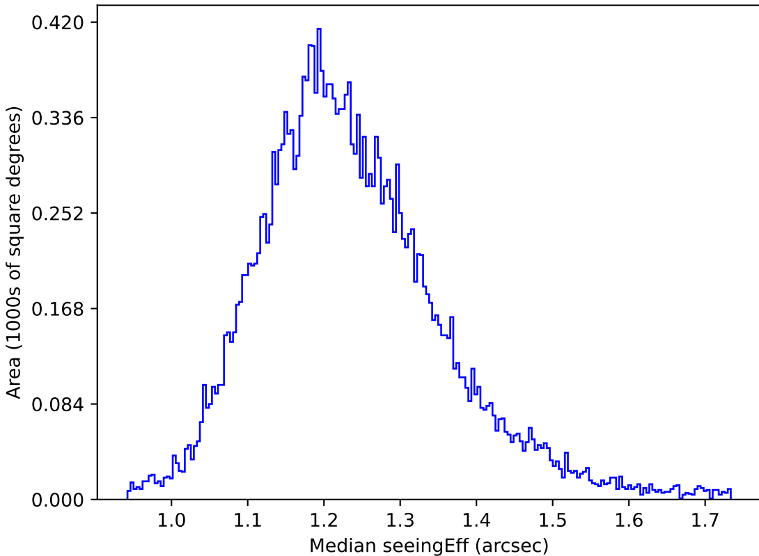
mw_roll_bulge_v3.3_10yrs All sky u band: Median seeingEff
