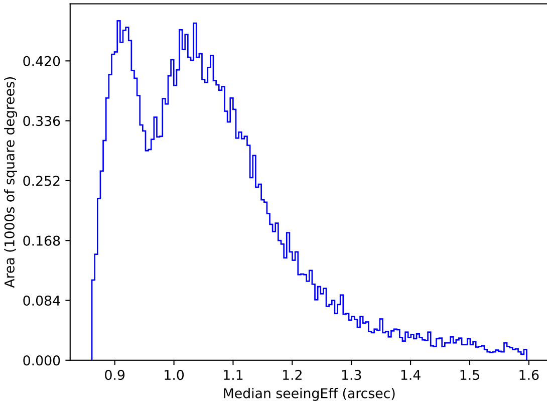
mw_roll_bulge_v3.3_10yrs All sky r band: Median seeingEff
