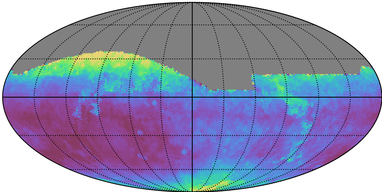
mw_roll_bulge_v3.3_10yrs All sky i band: Median seeingEff
