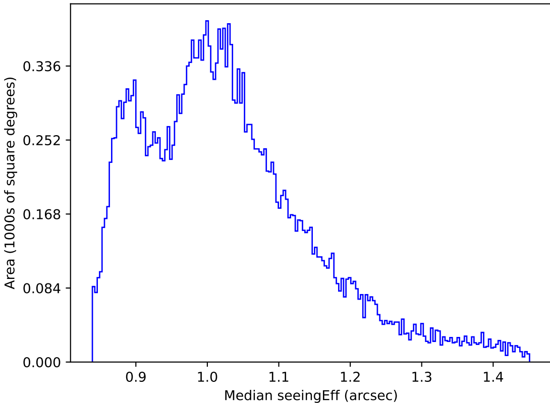
mw_roll_bulge_v3.3_10yrs All sky i band: Median seeingEff
