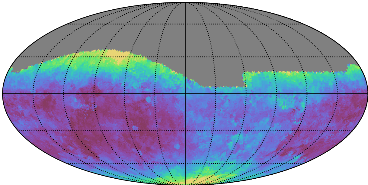
mw_roll_bulge_v3.3_10yrs All sky g band: Median seeingEff
