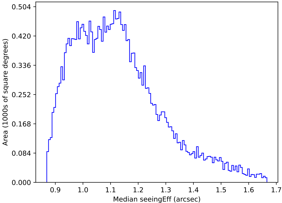
mw_roll_bulge_v3.3_10yrs All sky g band: Median seeingEff
