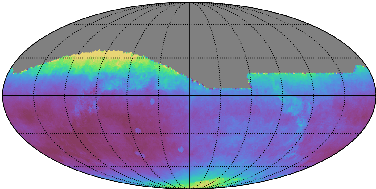
mw_roll_bulge_v3.3_10yrs All sky all bands: Median seeingEff
