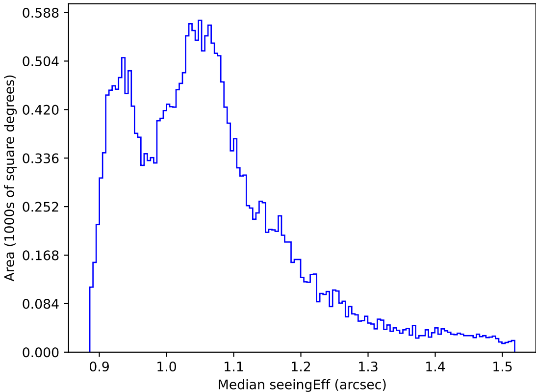
mw_roll_bulge_v3.3_10yrs All sky all bands: Median seeingEff
