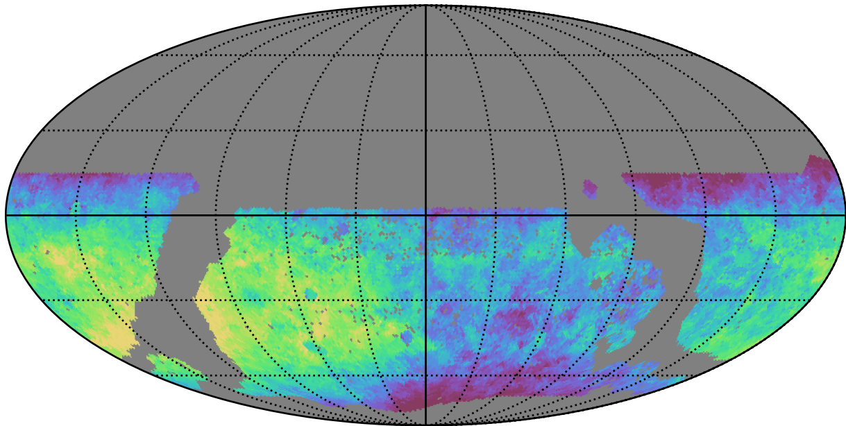
mw_roll_bulge_v3.3_10yrs WFD z band: Median saturation_mag
