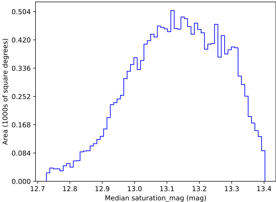
mw_roll_bulge_v3.3_10yrs WFD y band: Median saturation_mag
