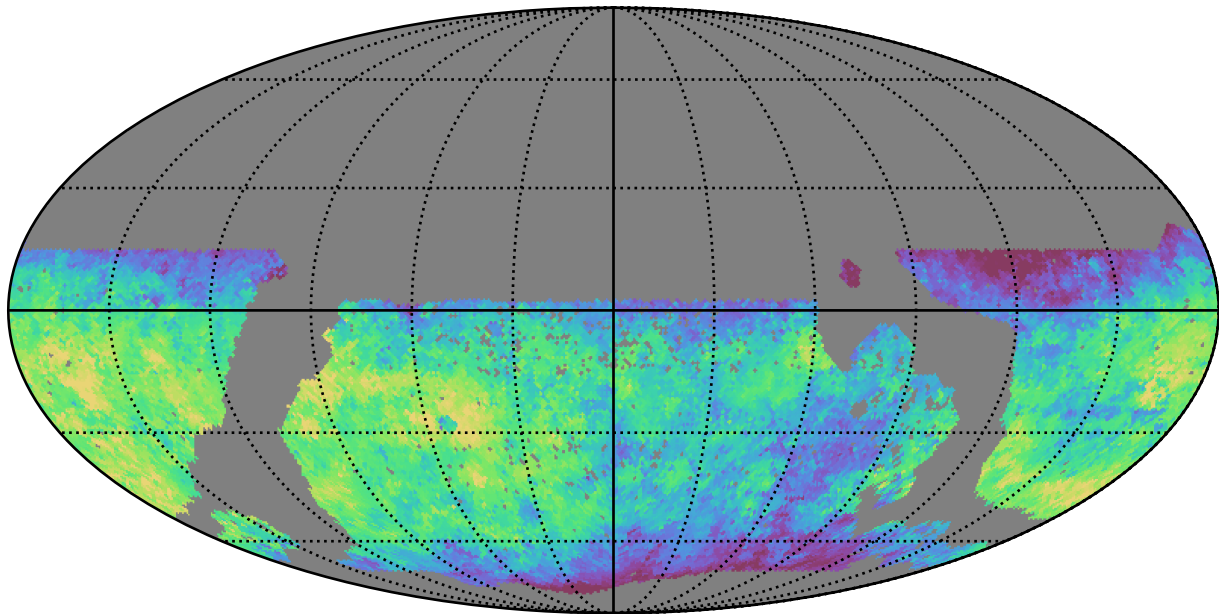
mw_roll_bulge_v3.3_10yrs WFD u band: Median saturation_mag
