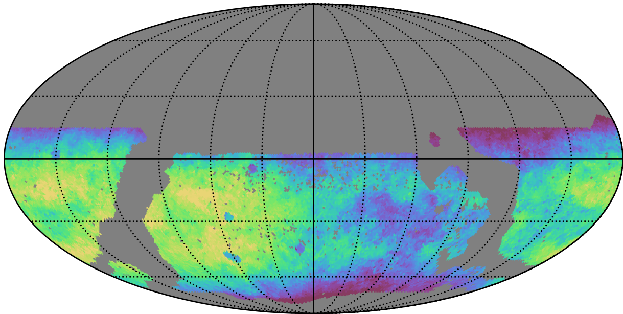
mw_roll_bulge_v3.3_10yrs WFD r band: Median saturation_mag
