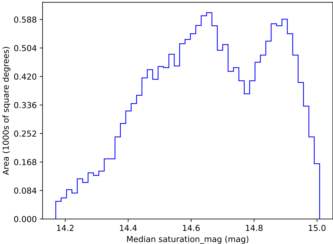
mw_roll_bulge_v3.3_10yrs WFD r band: Median saturation_mag
