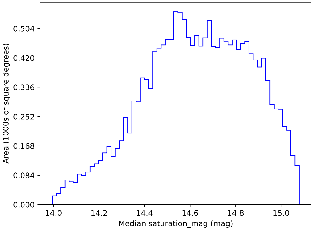
mw_roll_bulge_v3.3_10yrs WFD g band: Median saturation_mag
