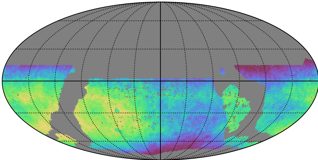
mw_roll_bulge_v3.3_10yrs WFD all bands: Median saturation_mag
