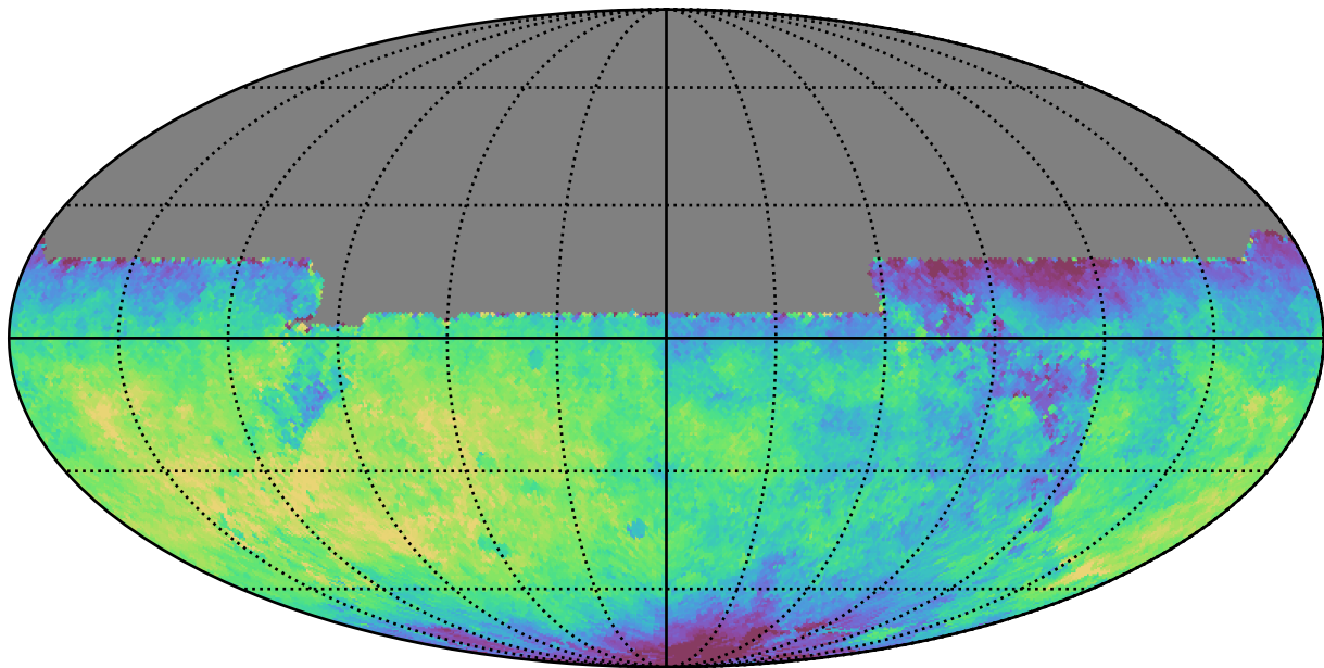
mw_roll_bulge_v3.3_10yrs All sky y band: Median saturation_mag
