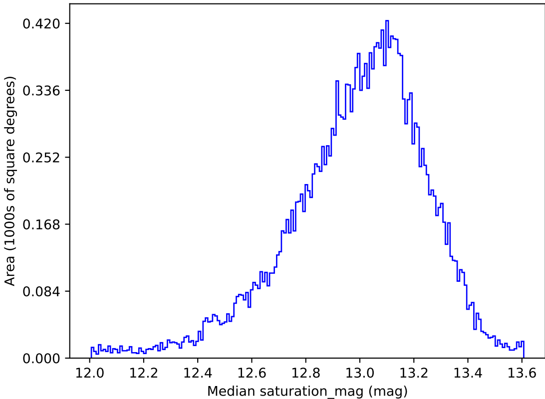
mw_roll_bulge_v3.3_10yrs All sky u band: Median saturation_mag
