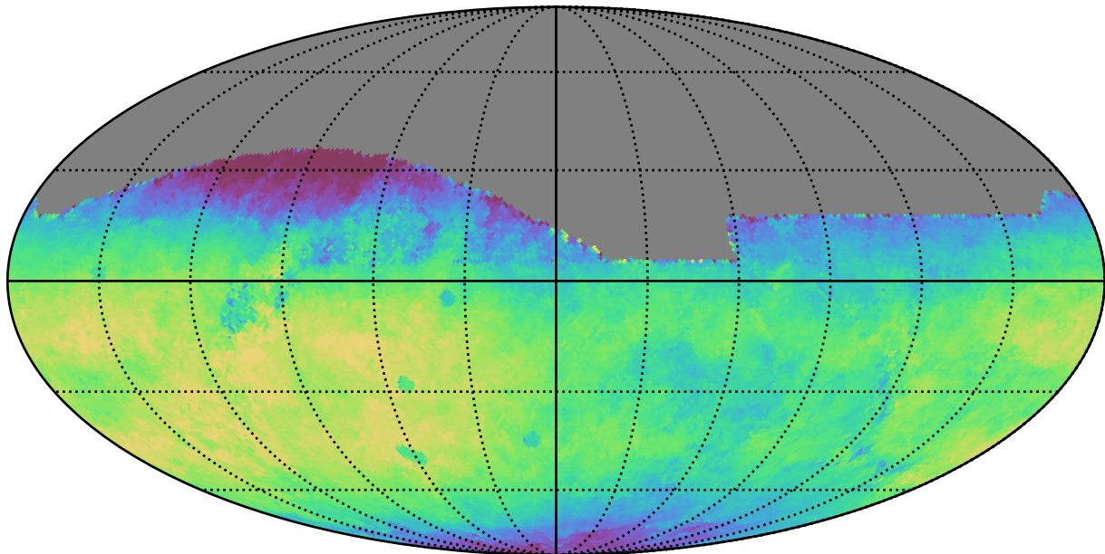
mw_roll_bulge_v3.3_10yrs All sky r band: Median saturation_mag
