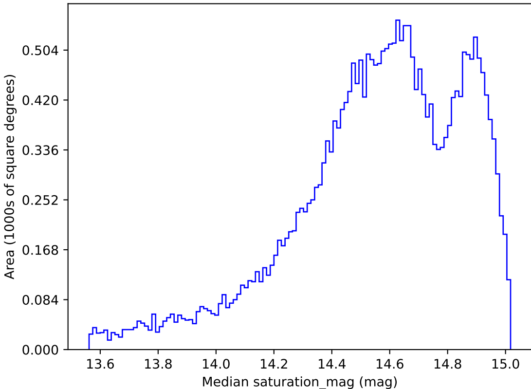
mw_roll_bulge_v3.3_10yrs All sky r band: Median saturation_mag
