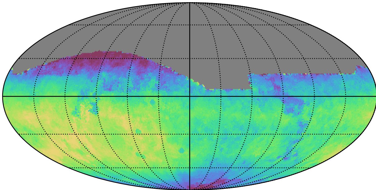
mw_roll_bulge_v3.3_10yrs All sky i band: Median saturation_mag
