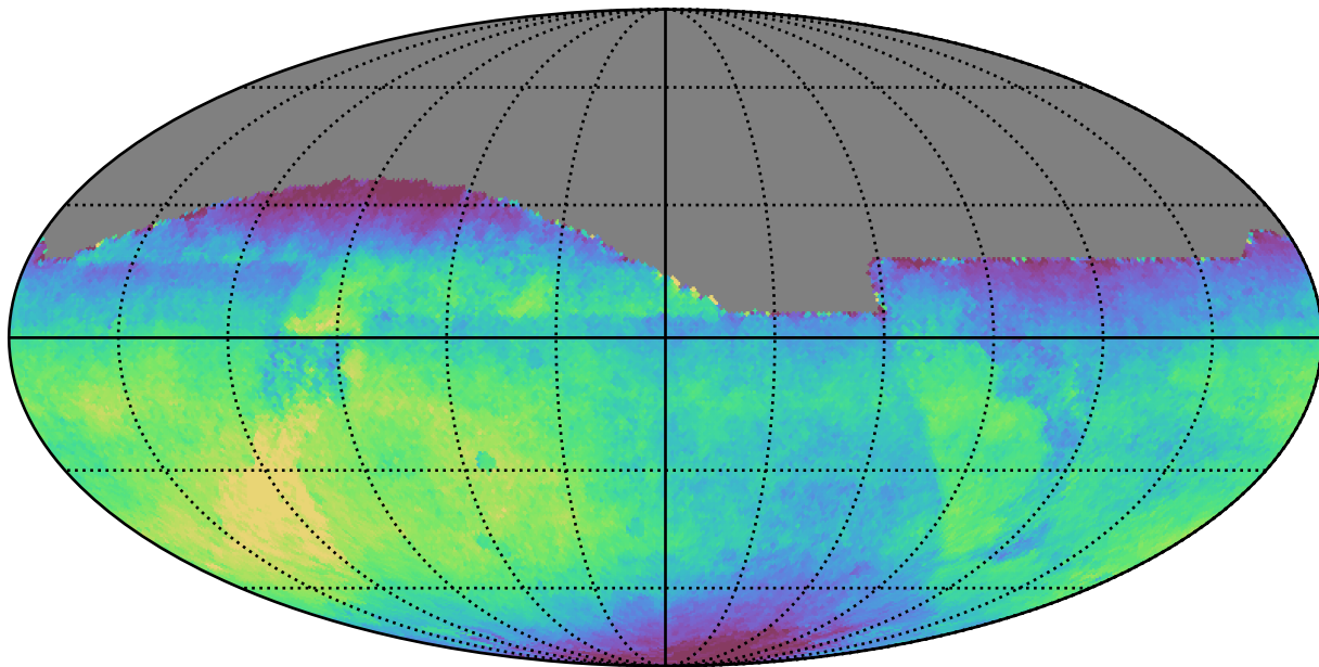
mw_roll_bulge_v3.3_10yrs All sky all bands: Median saturation_mag
