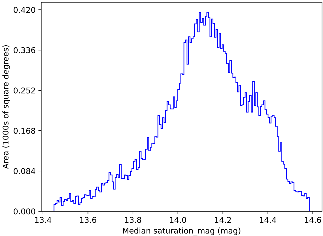
mw_roll_bulge_v3.3_10yrs All sky all bands: Median saturation_mag
