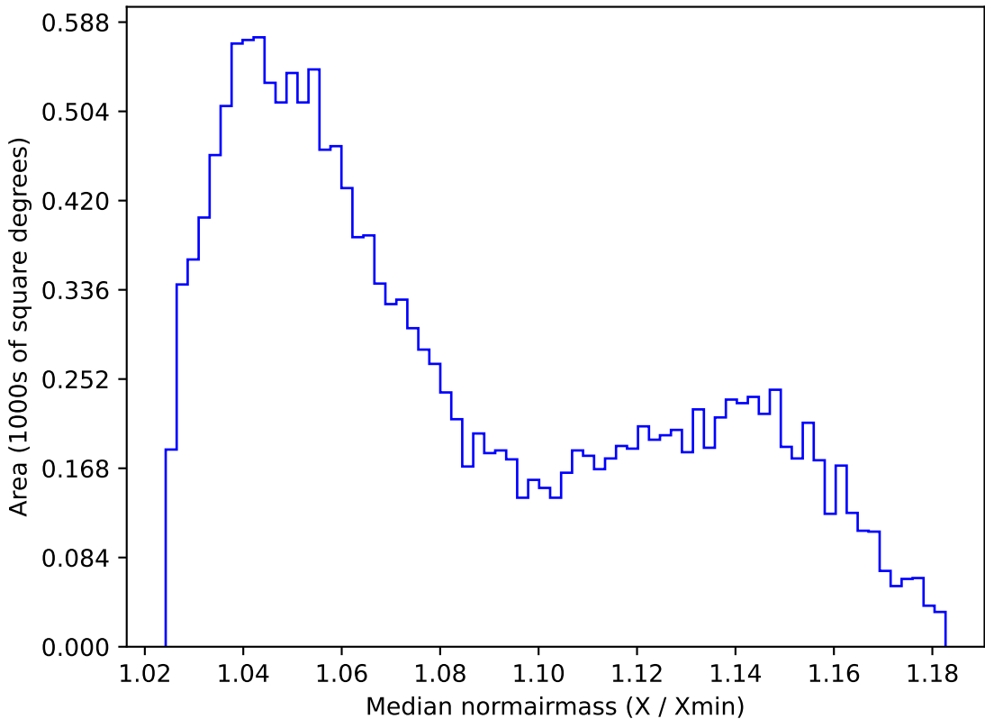
mw_roll_bulge_v3.3_10yrs WFD z band: Median normairmass
