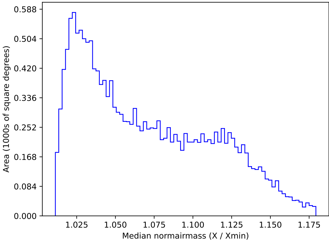
mw_roll_bulge_v3.3_10yrs WFD u band: Median normairmass
