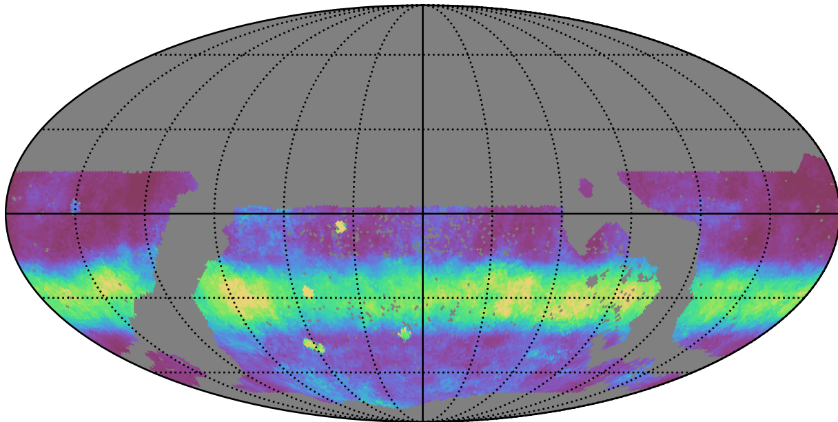
mw_roll_bulge_v3.3_10yrs WFD r band: Median normairmass
