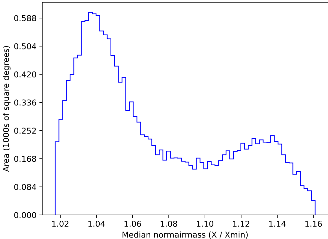
mw_roll_bulge_v3.3_10yrs WFD i band: Median normairmass
