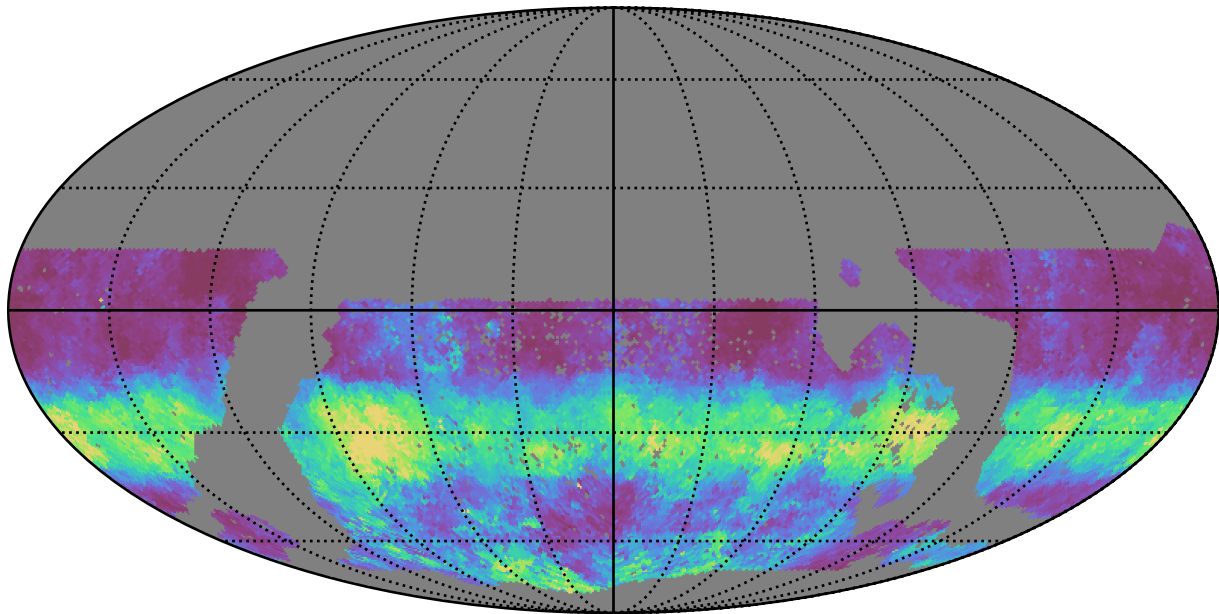
mw_roll_bulge_v3.3_10yrs WFD g band: Median normairmass
