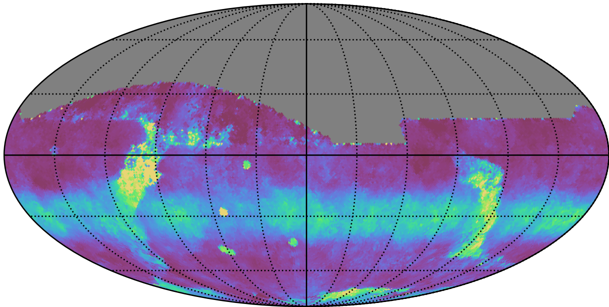
mw_roll_bulge_v3.3_10yrs All sky z band: Median normairmass
