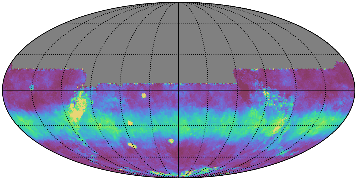
mw_roll_bulge_v3.3_10yrs All sky y band: Median normairmass
