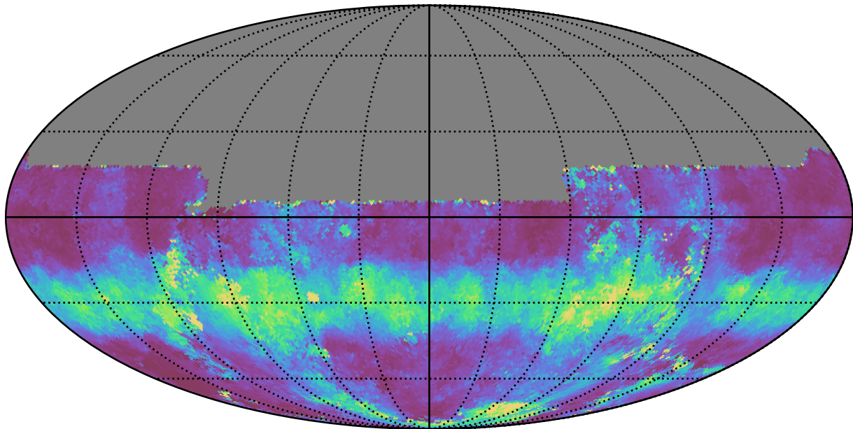
mw_roll_bulge_v3.3_10yrs All sky u band: Median normairmass
