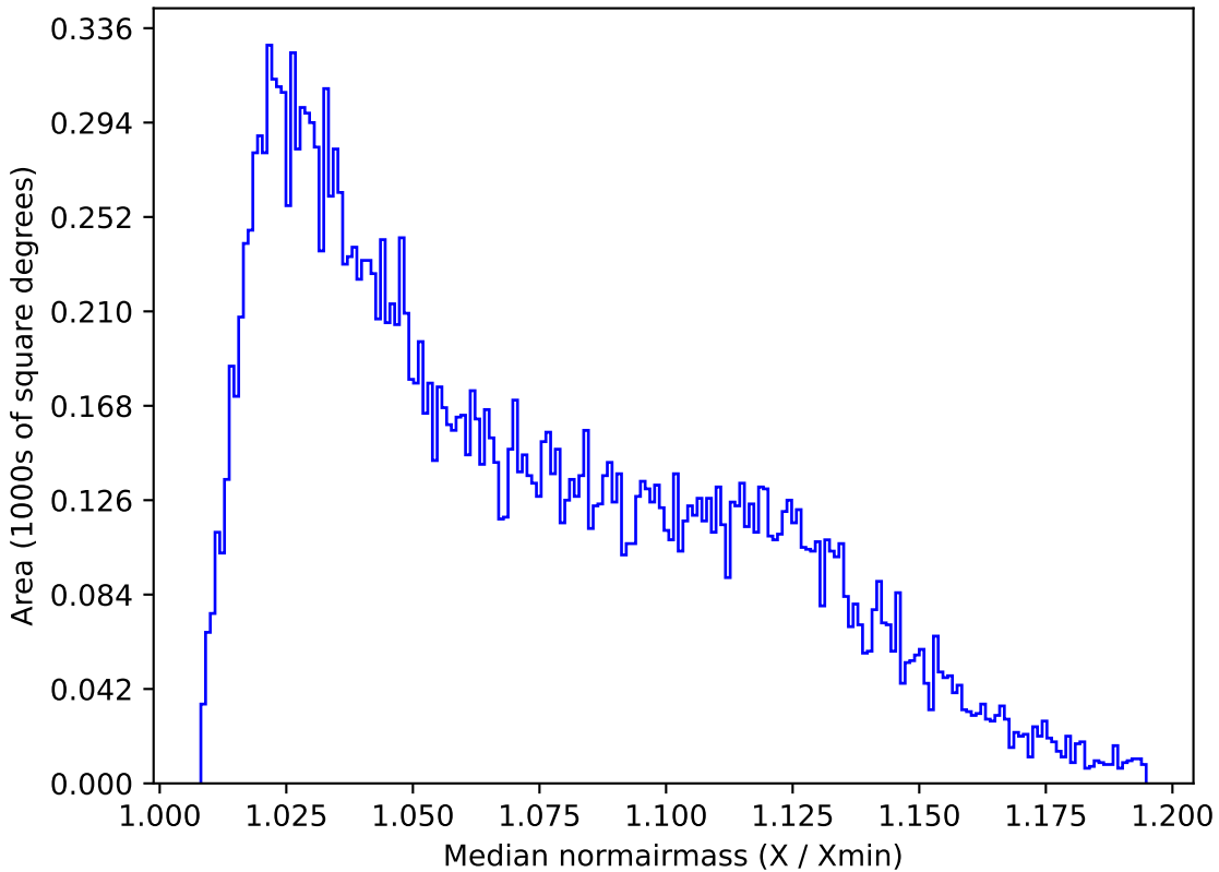
mw_roll_bulge_v3.3_10yrs All sky u band: Median normairmass
