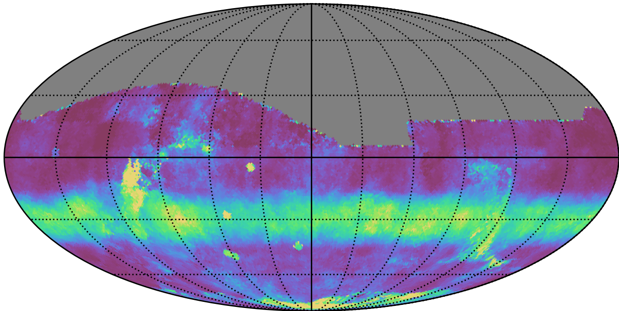
mw_roll_bulge_v3.3_10yrs All sky r band: Median normairmass
