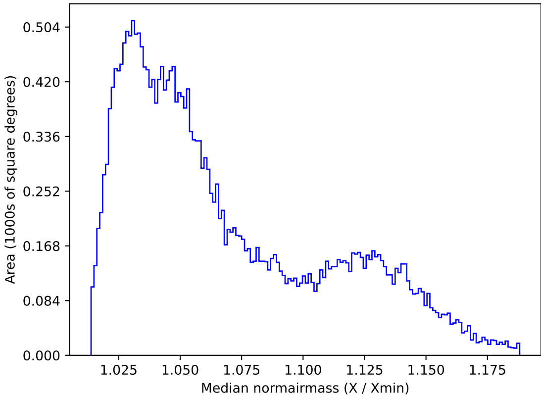
mw_roll_bulge_v3.3_10yrs All sky r band: Median normairmass
