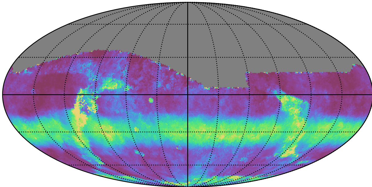
mw_roll_bulge_v3.3_10yrs All sky i band: Median normairmass
