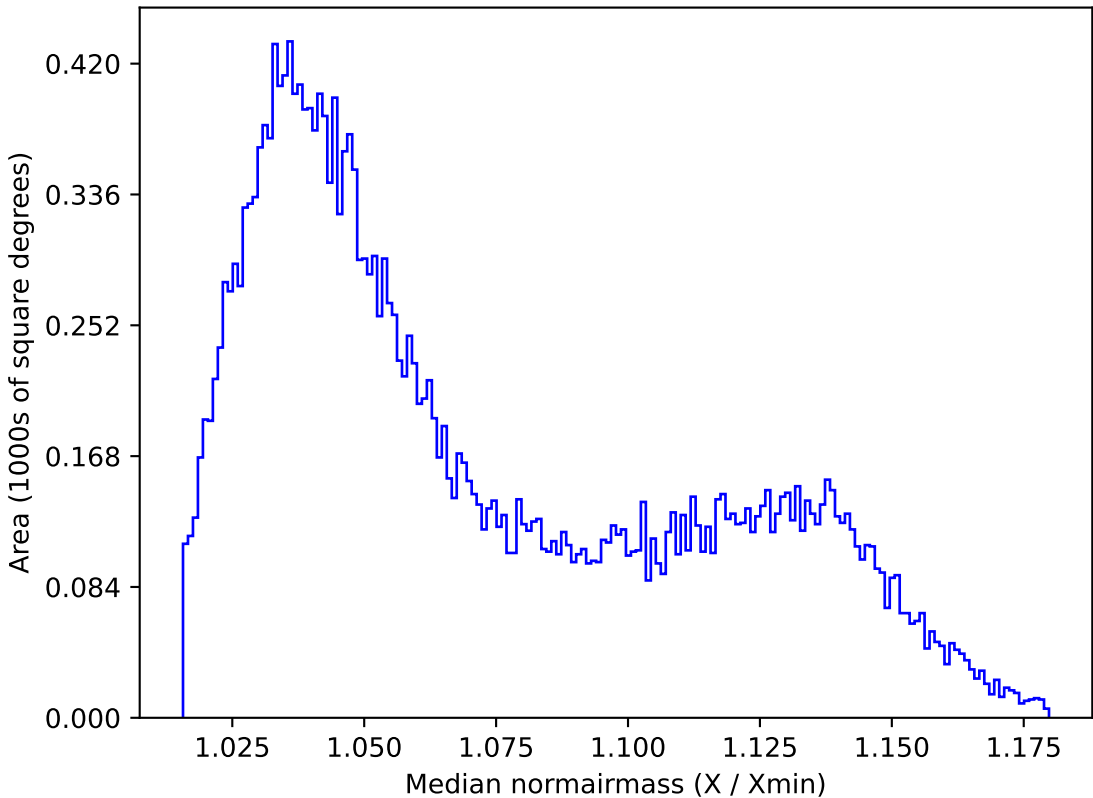
mw_roll_bulge_v3.3_10yrs All sky i band: Median normairmass
