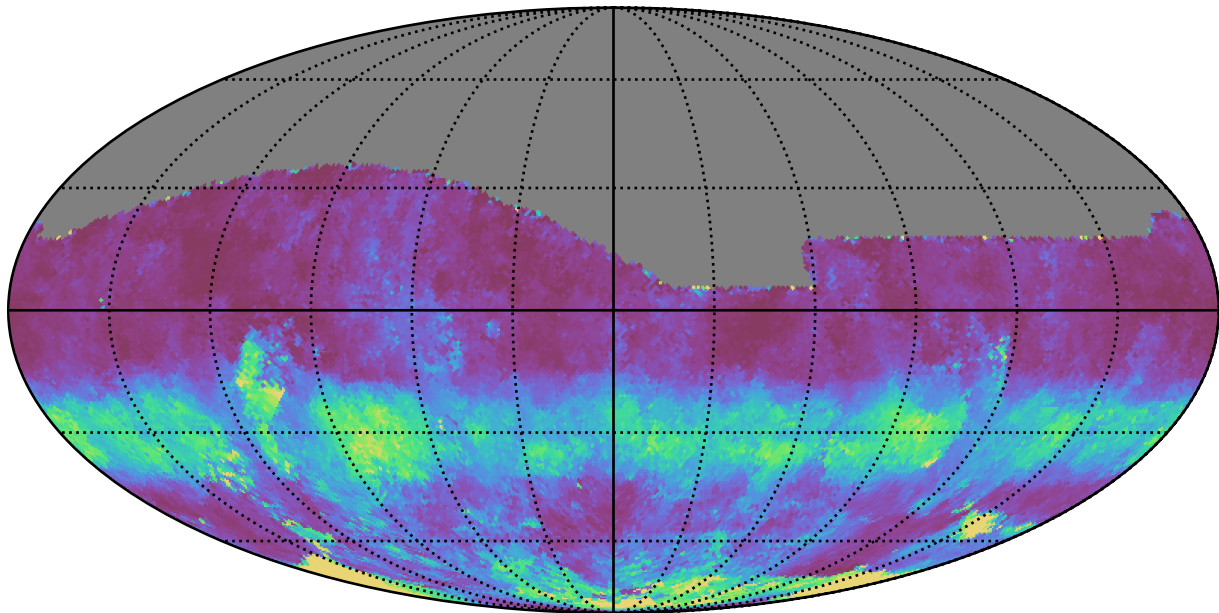
mw_roll_bulge_v3.3_10yrs All sky g band: Median normairmass
