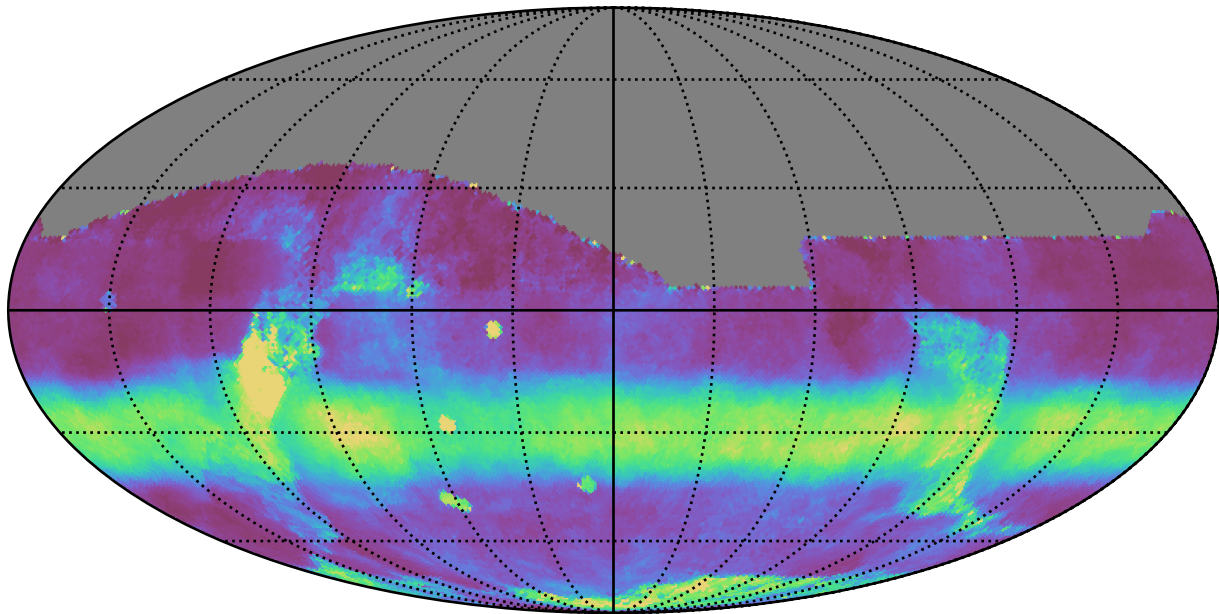
mw_roll_bulge_v3.3_10yrs All sky all bands: Median normairmass
