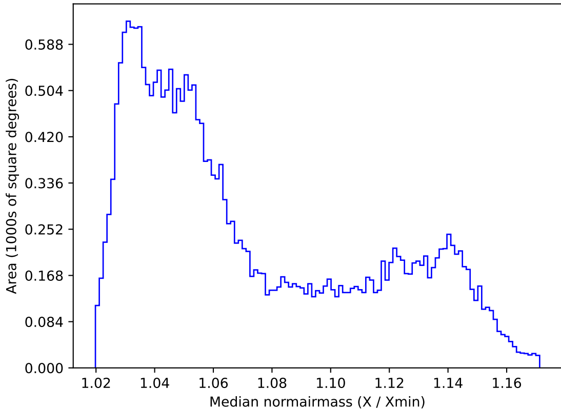
mw_roll_bulge_v3.3_10yrs All sky all bands: Median normairmass
