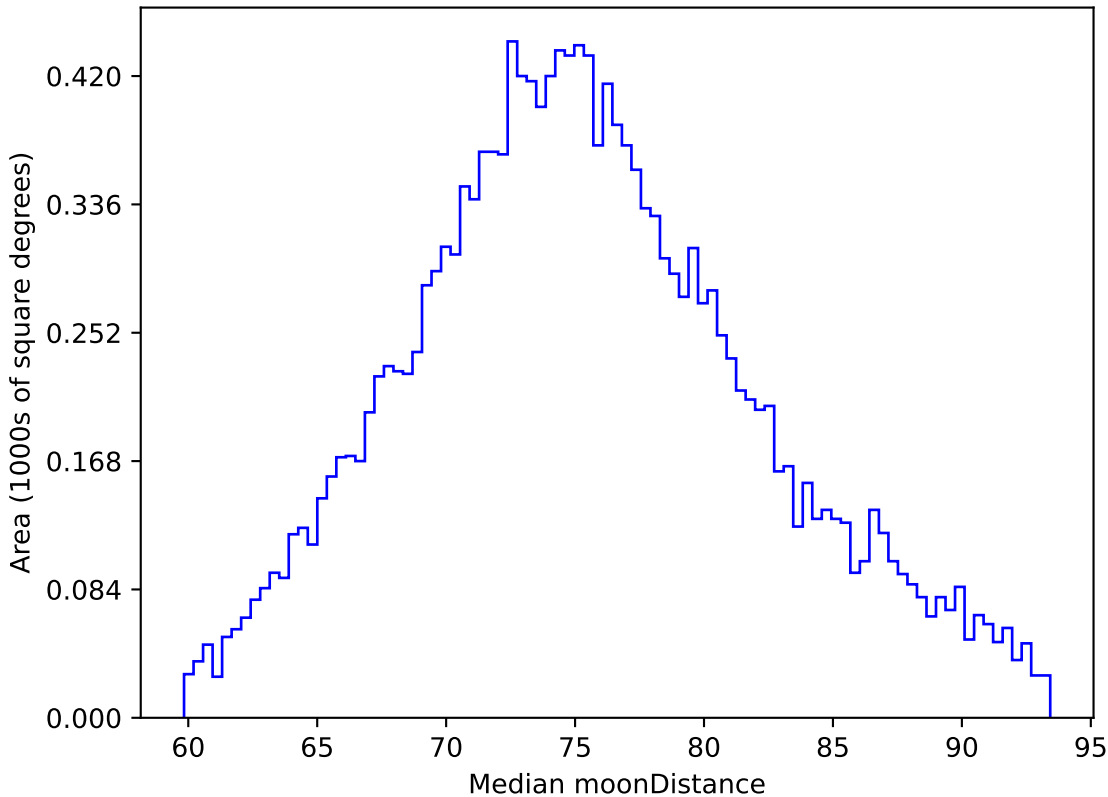
mw_roll_bulge_v3.3_10yrs WFD z band: Median moonDistance
