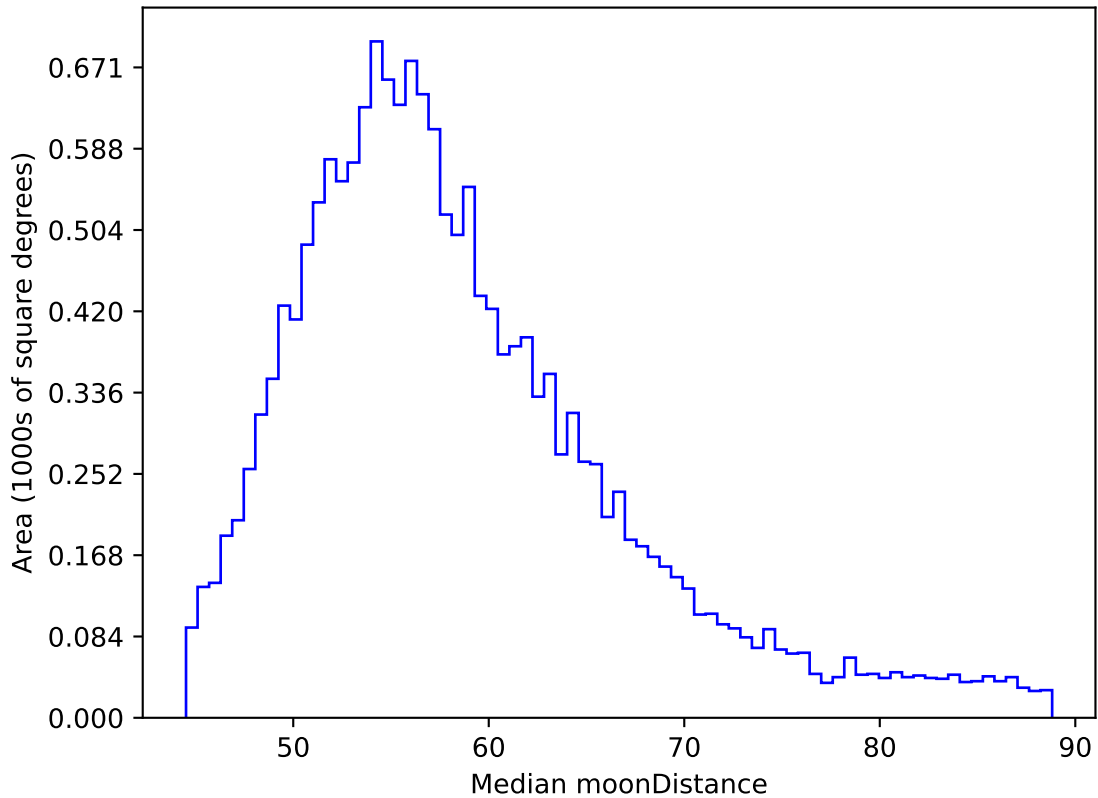
mw_roll_bulge_v3.3_10yrs WFD y band: Median moonDistance
