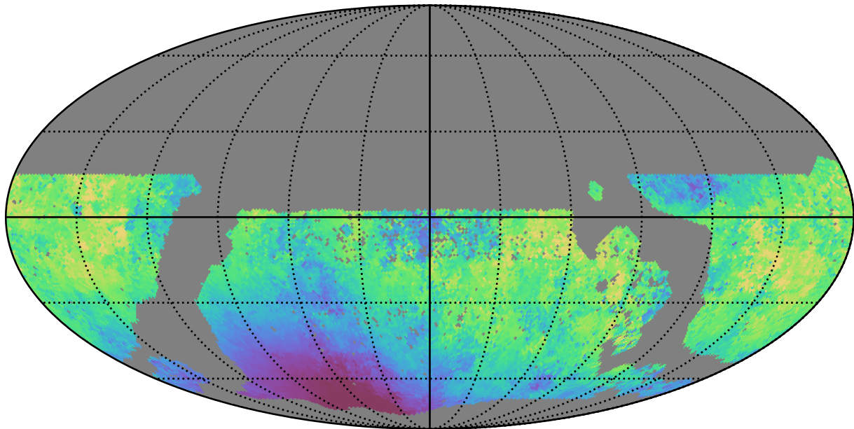
mw_roll_bulge_v3.3_10yrs WFD u band: Median moonDistance
