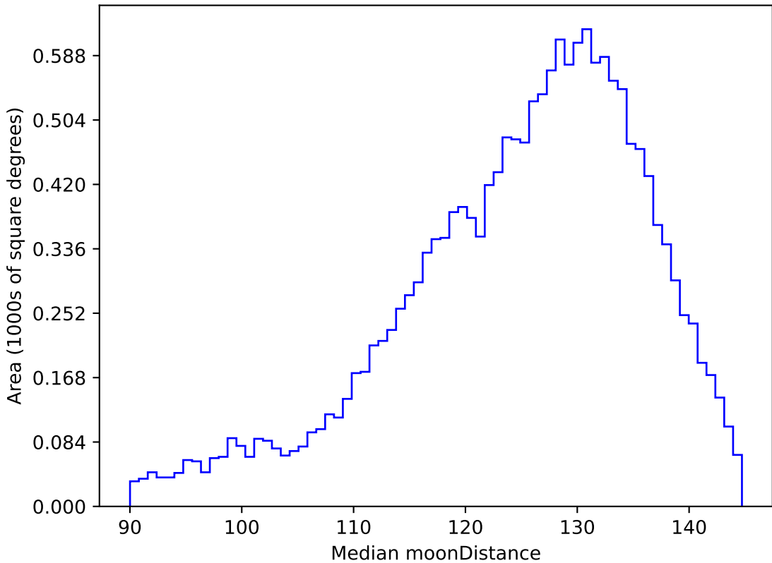
mw_roll_bulge_v3.3_10yrs WFD u band: Median moonDistance
