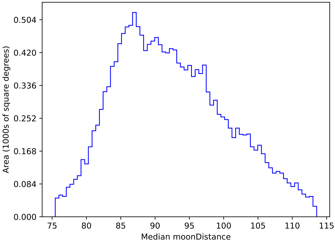
mw_roll_bulge_v3.3_10yrs WFD i band: Median moonDistance
