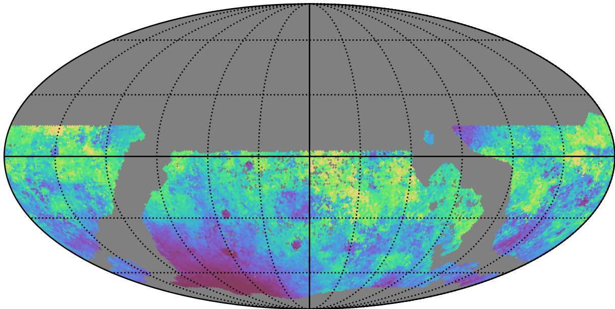
mw_roll_bulge_v3.3_10yrs WFD g band: Median moonDistance
